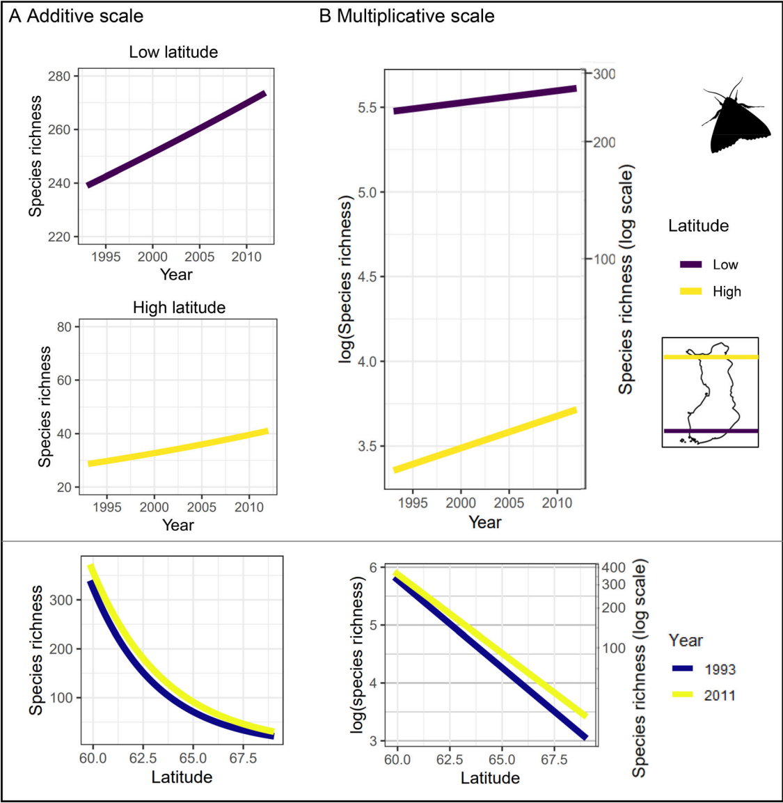
Fig. 5. Top: predicted changes in site-level species richness of moths over time at low (61°, purple) and high (68°, yellow) latitudes in Finland, plotted on (A) additive and (B) multiplicative scales. On the additive scale, the rate of species-richness change over time – the slope of the lines – is stronger at low latitudes (purple line), where sites experienced higher gains in the absolute numbers of species during the monitoring period. By contrast, the rate of richness increases is greatest at high latitudes when presented on the logarithmic scale (yellow line), corresponding to the scale of measurement of a generalised linear mixed model applied to species counts. Bottom: Predicted changes in site-level species richness across latitude shown for 2 years. Data from Antão et al. (2020).
