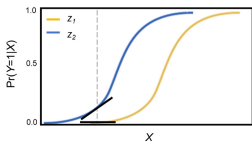
Fig. 3. Predicted probabilities of Y ( \Pr(Y=1) ) obtained from a logistic regression model with continuous X and Z predictors and no statistical interaction. The marginal effect of X is shown at the vertical dashed line by the slope of the tangent to the S-shaped curve.
